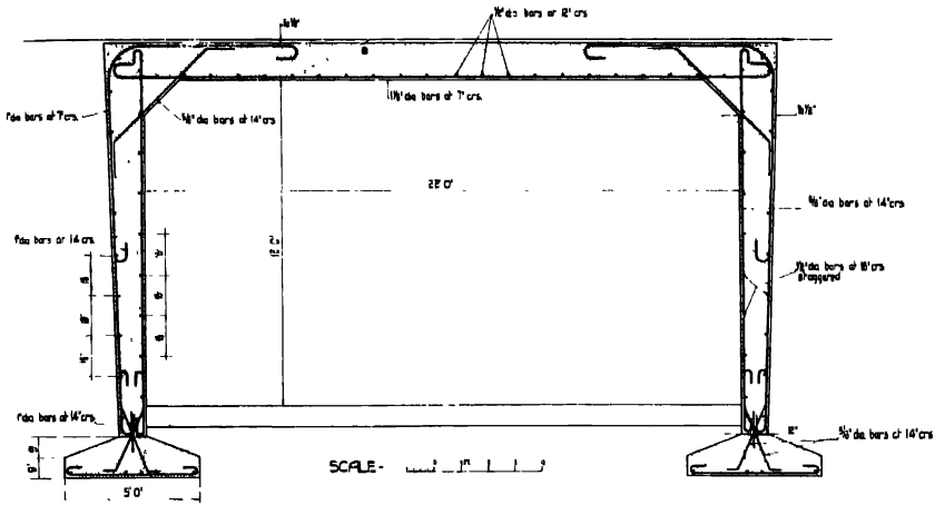
Fig. 119.—Arrangement of Reinforcement.
